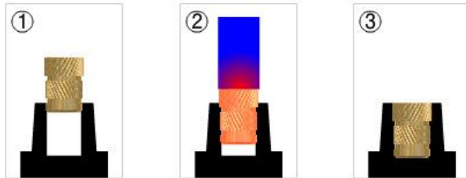
①Set insert nut→②Termocompression→③Complete
